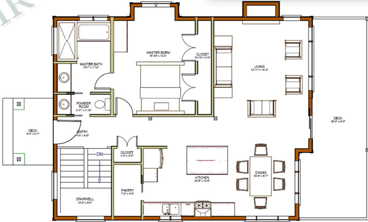
MAIN FLOOR 1140 sq ft
