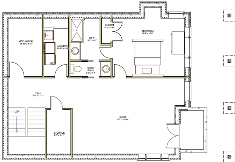
LOWER FLOOR 1125 sq ft
