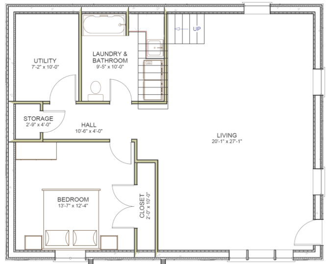
LOWER FLOOR 1060 sq ft
